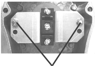
Adjusting screw for calibrating switching point
